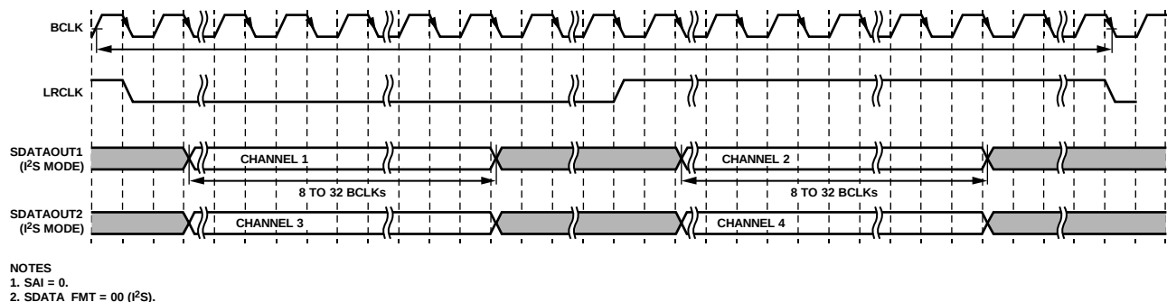
Figure 22. I 2 S Audio Format
